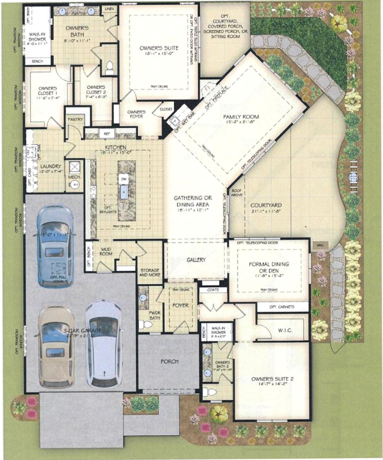
FIRST FLOOR RANCH
