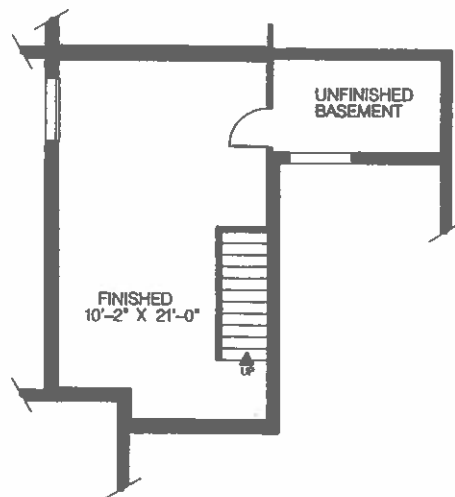
BASEMENT PLAN
